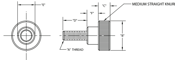
Knurled-Type Thumb Screws with Shoulder
